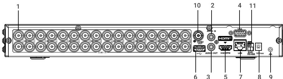
Description of Rear Panel
